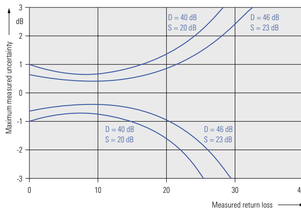
Maximum measurement uncertainty for a return loss S of 20 dB and 23 dB at the test port and directivity D of 40 dB and 46 dB
